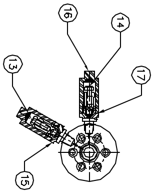
SECTION THROUGH GLAND AT FITTINGS (NOT TO SCALE)
